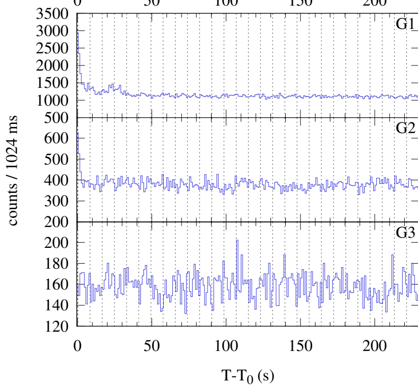
Konus-WIND S2 SOL2022-08-27T09:15 (C4.4) T_0 = 33342.306 s UT (09:15:42.306)
