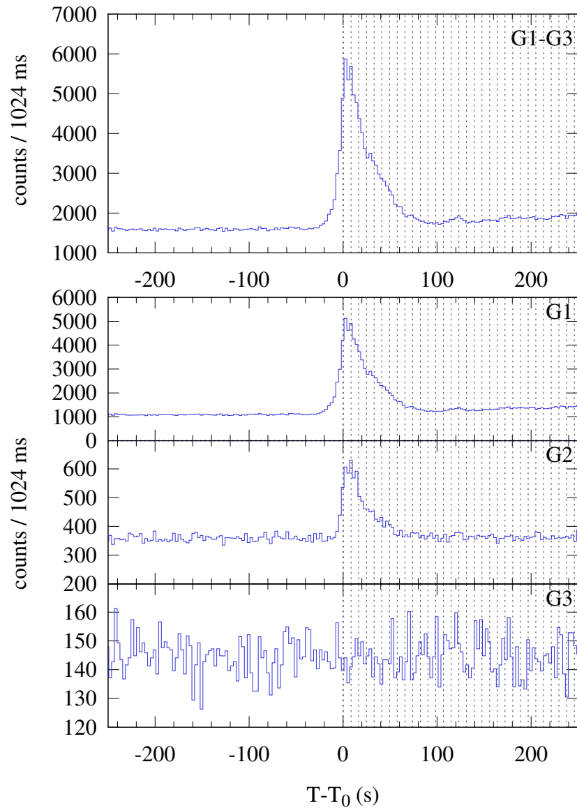
Konus-WIND S2 SOL2022-10-01T20:03 (M5.8) T_0 = 72188.150 s UT (20:03:08.150)
