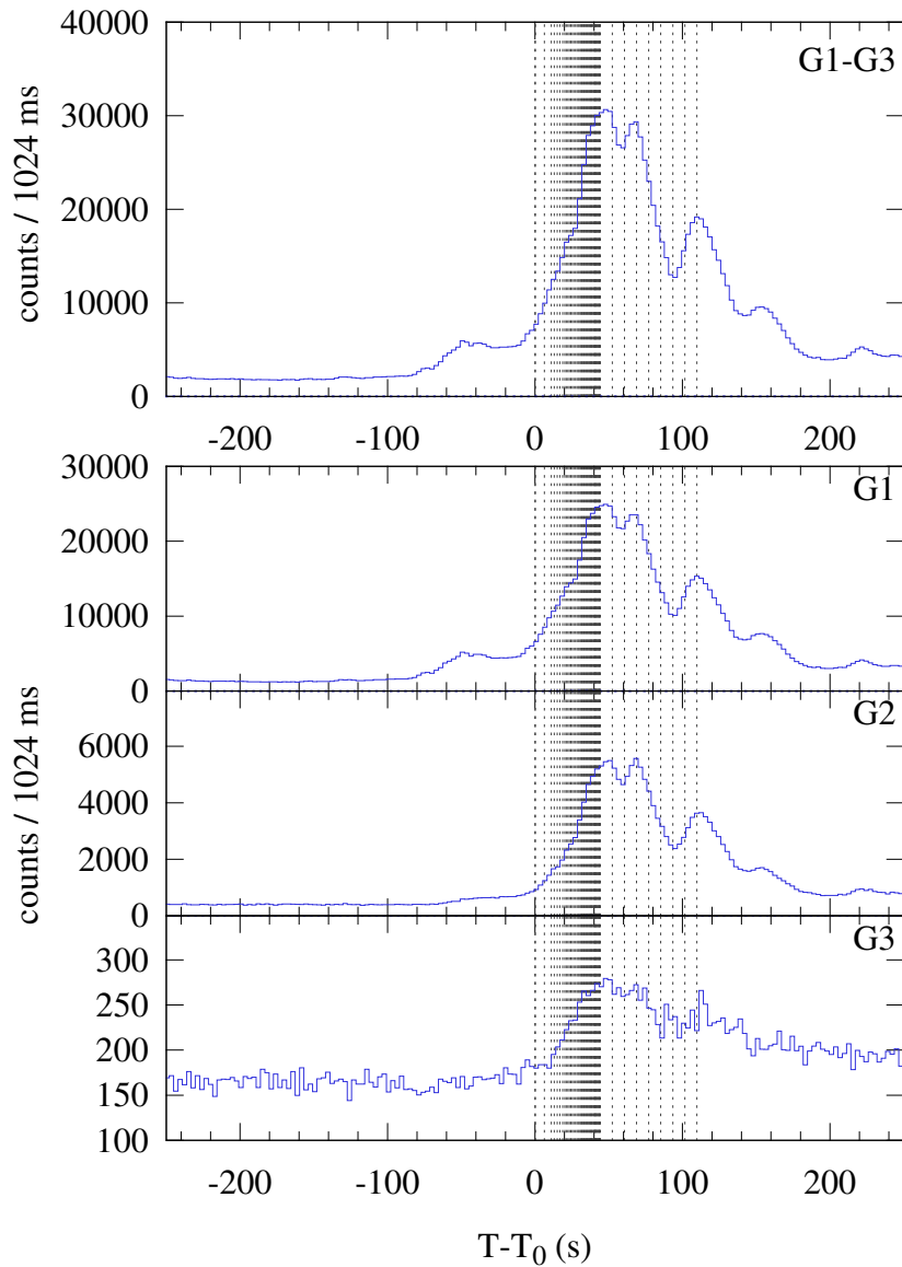
Konus-WIND S2 SOL2022-10-02T20:21 (X1.0) T_0 = 73264.926 s UT (20:21:04.926)
