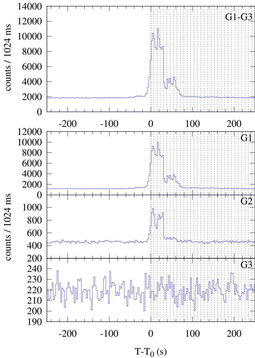
Konus-WIND S2 SOL2022-10-11T10:50 (M1.5) T_0 = 39046.971 s UT (10:50:46.971)
