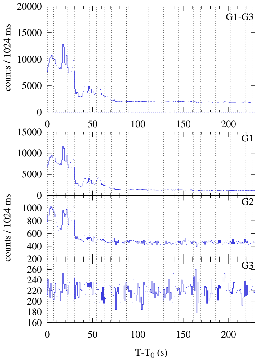
Konus-WIND S2 SOL2022-10-11T10:50 (M1.5) T_0 = 39046.971 s UT (10:50:46.971)
