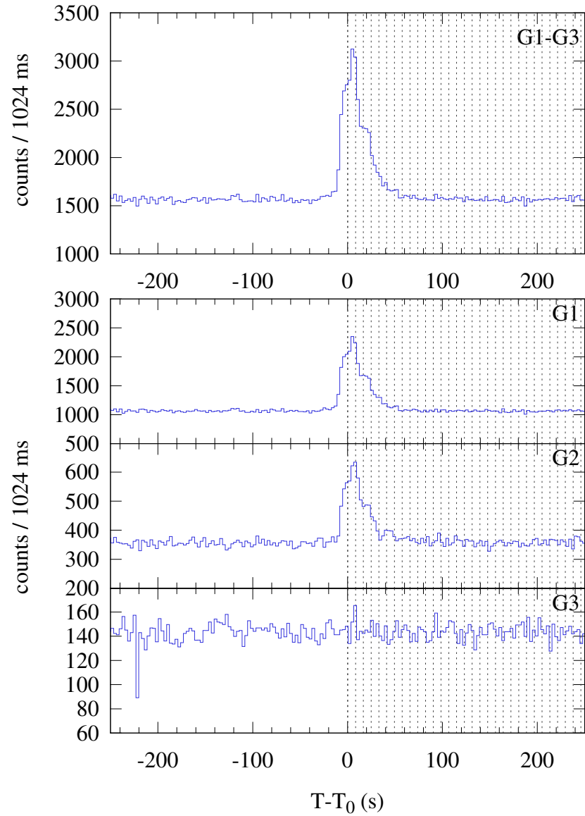
Konus-WIND S2 SOL2023-04-17T06:32 (C7.0) T_0 = 23561.342 s UT (06:32:41.342)
