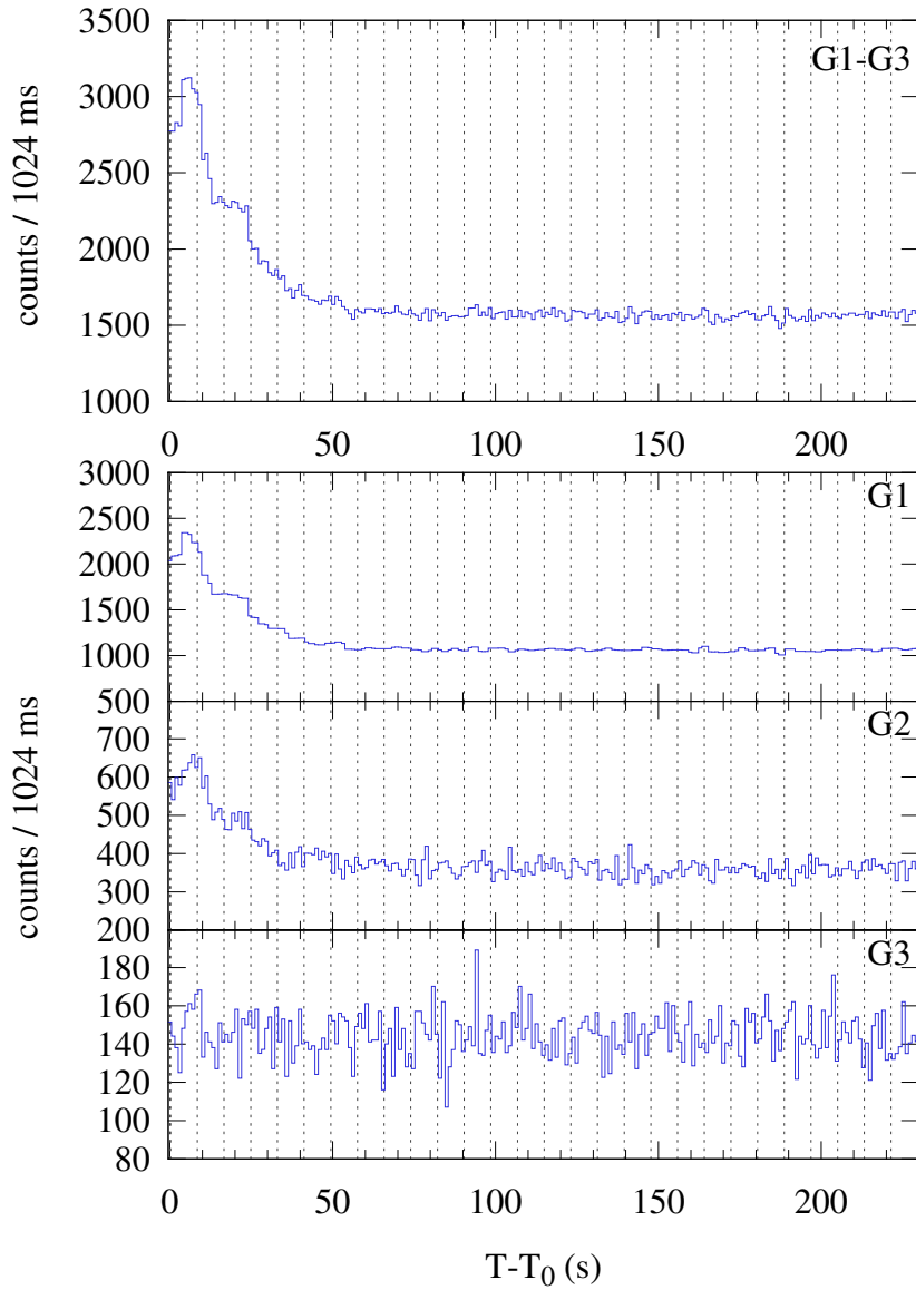
Konus-WIND S2 SOL2023-04-17T06:32 (C7.0) T_0 = 23561.342 s UT (06:32:41.342)
