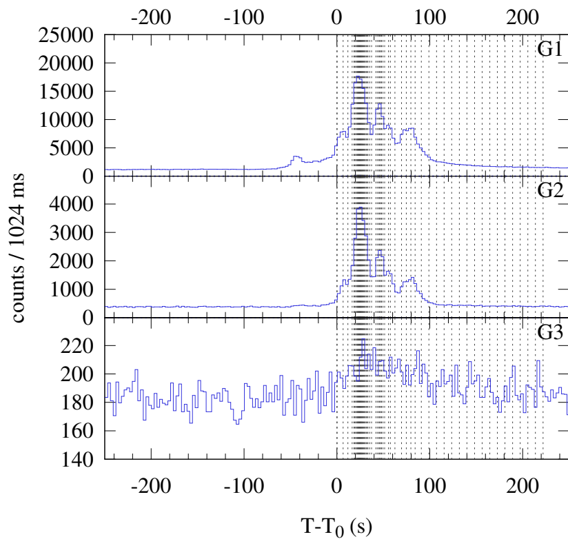
Konus-WIND S2 SOL2023-05-09T03:51 (M6.5) T_0 = 13877.921 s UT (03:51:17.921)
