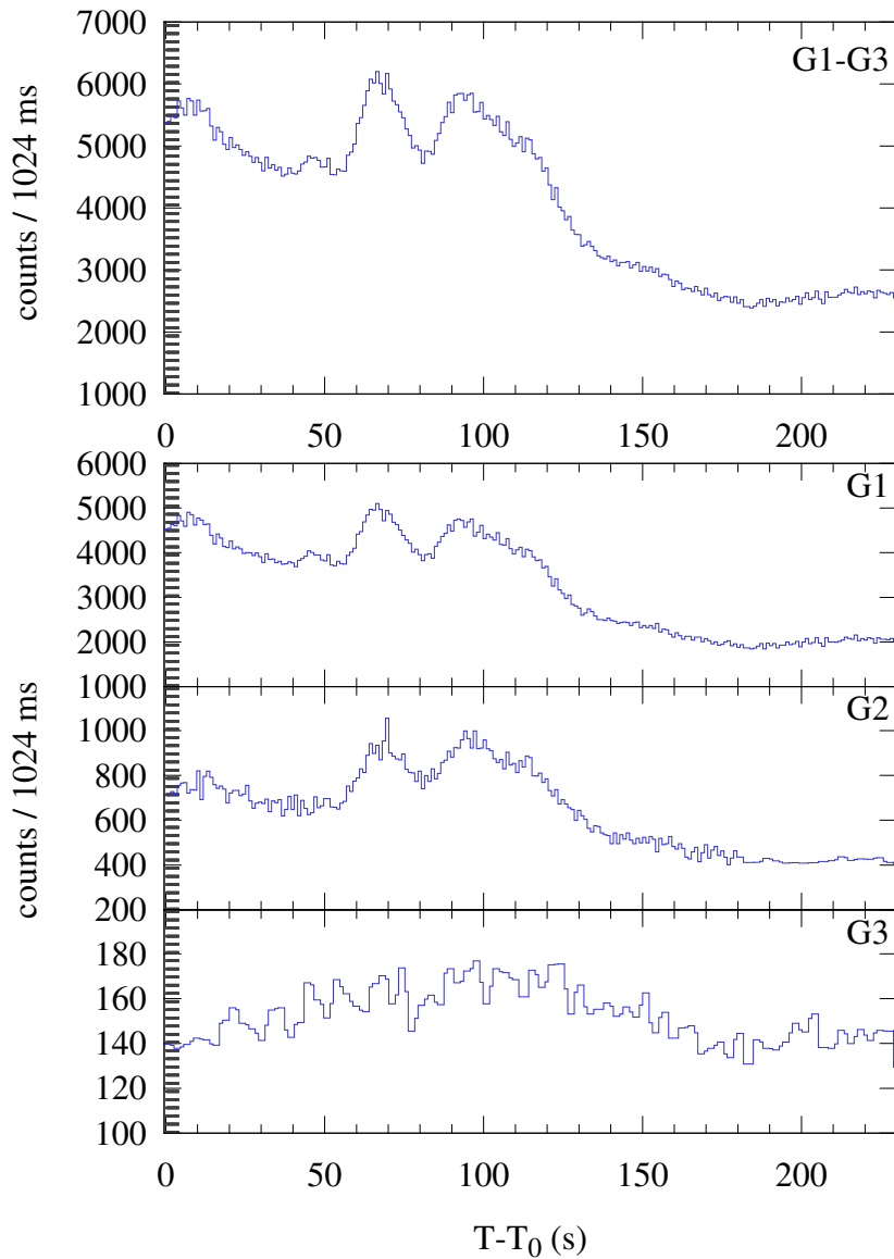
Konus-WIND S2 SOL2023-06-20T17:05 (X1.1) T_0 = 61557.671 s UT (17:05:57.671)
