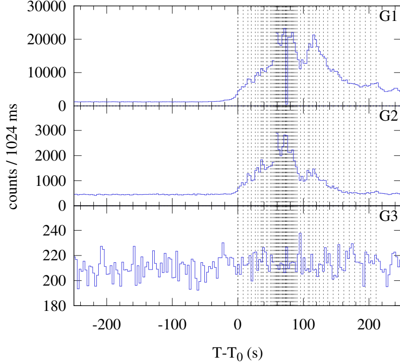
Konus-WIND S2 SOL2023-07-16T17:38 (M4.0) T_0 = 63525.491 s UT (17:38:45.491)
