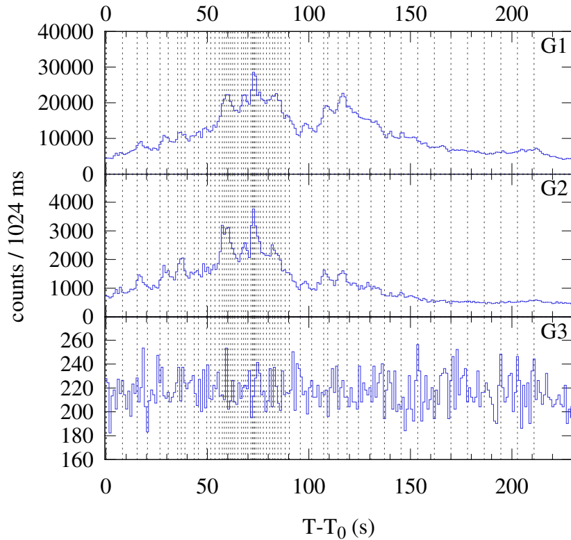
Konus-WIND S2 SOL2023-07-16T17:38 (M4.0) T_0 = 63525.491 s UT (17:38:45.491)
