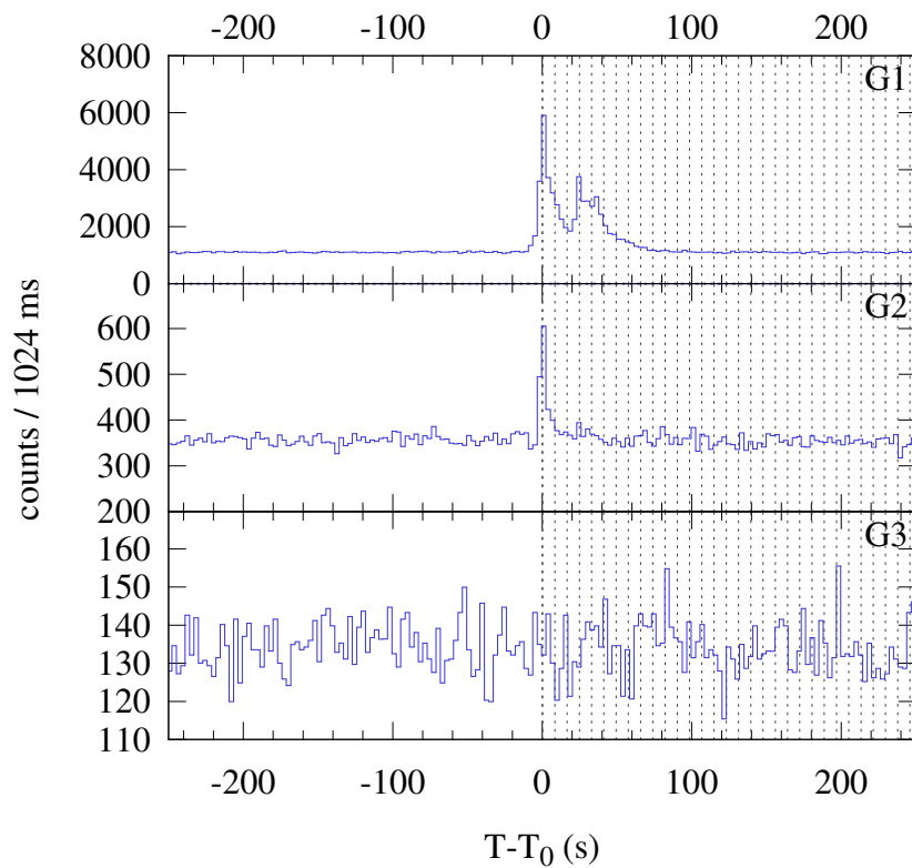
Konus-WIND S2 SOL2023-08-02T14:51 (M1.7) T_0 = 53469.142 s UT (14:51:09.142)
