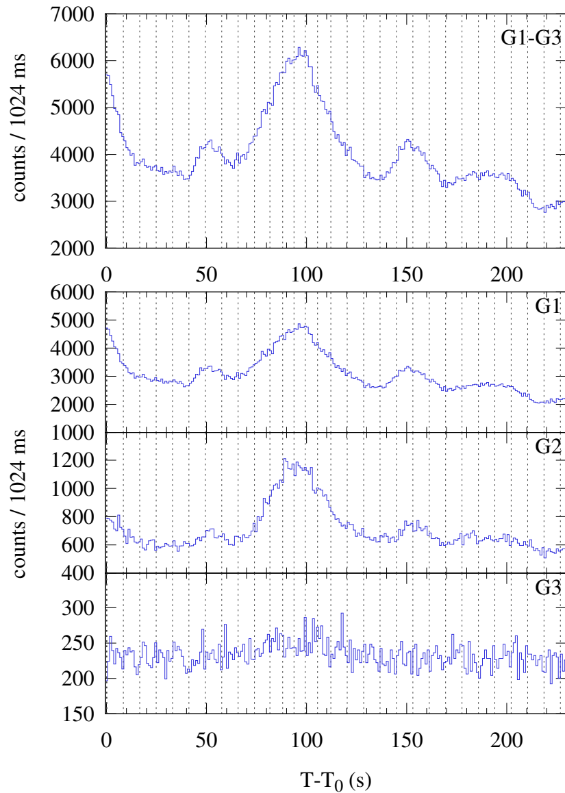
Konus-WIND S2 SOL2023-08-06T18:31 (M5.5) T_0 = 66706.901 s UT (18:31:46.901)
