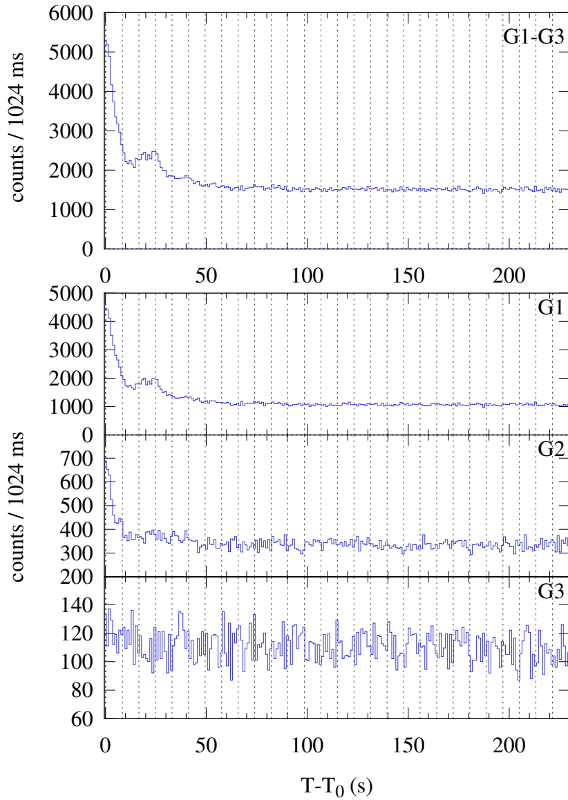
Konus-WIND S2 SOL2023-09-28T09:06 (M1.2) T_0 = 32770.355 s UT (09:06:10.355)
