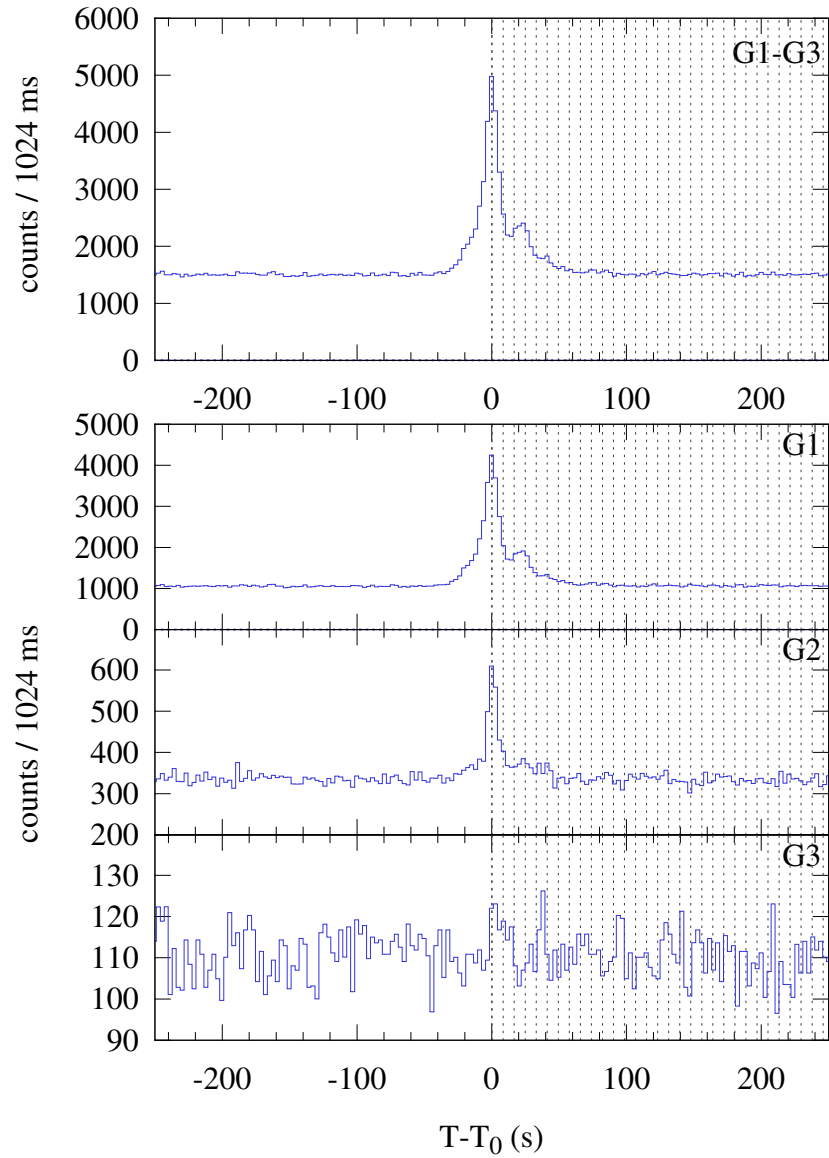
Konus-WIND S2 SOL2023-09-28T09:06 (M1.2) T_0 = 32770.355 s UT (09:06:10.355)
