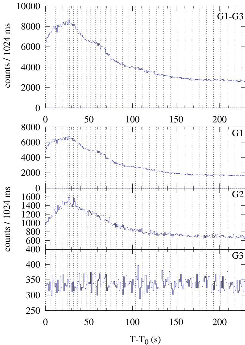
Konus-WIND S2 SOL2023-12-15T07:33 (M6.9) T_0 = 27215.148 s UT (07:33:35.148)
