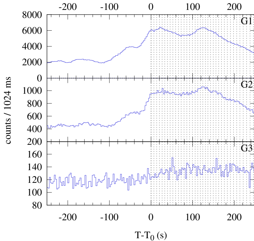
Konus-WIND S2 SOL2024-01-29T04:17 (M6.8) T_0 = 15434.50 s UT (04:17:14.50)
