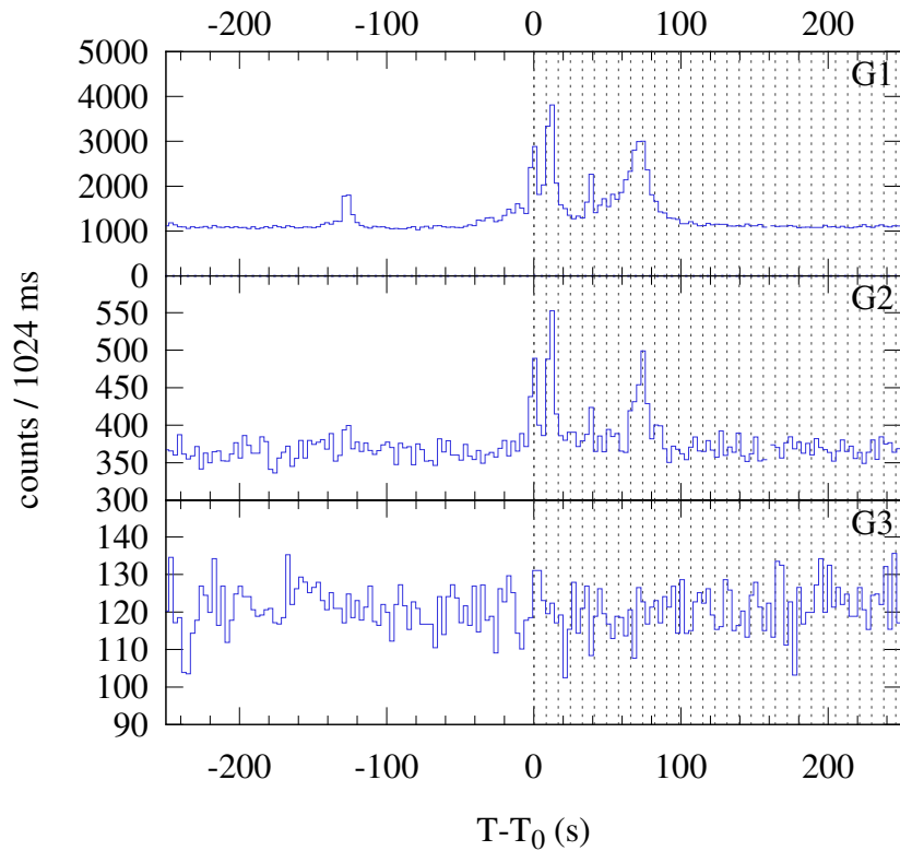
Konus-WIND S2 SOL2024-02-09T00:39 (M3.1) T_0 = 2378.255 s UT (00:39:38.255)
