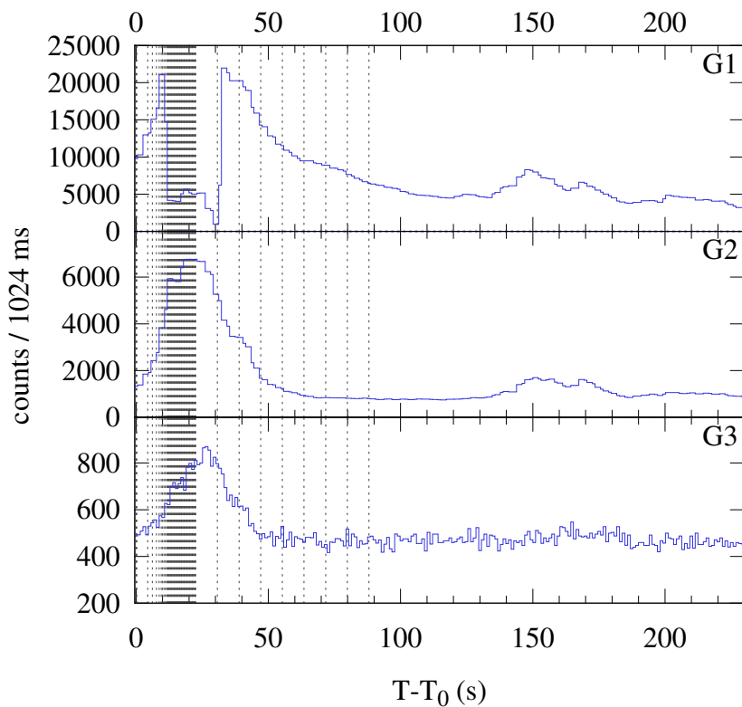
Konus-WIND S2 SOL2024-02-16T06:50 (X2.5) T_0 = 24654.592 s UT (06:50:54.592)
