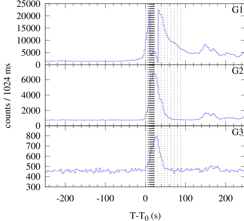
Konus-WIND S2 SOL2024-02-16T06:50 (X2.5) T_0 = 24654.592 s UT (06:50:54.592)
