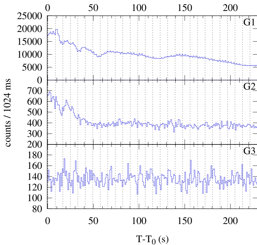
Konus-WIND S2 SOL2024-02-22T06:29 (X1.7) T_0 = 23351.413 s UT (06:29:11.413)
