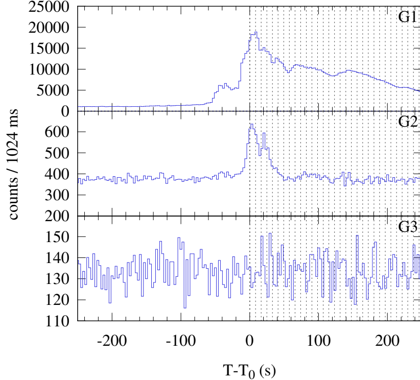
Konus-WIND S2 SOL2024-02-22T06:29 (X1.7) T_0 = 23351.413 s UT (06:29:11.413)
