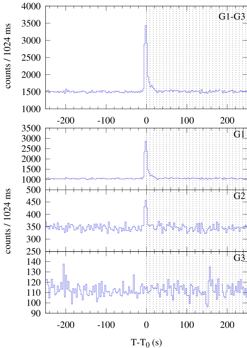
Konus-WIND S2 SOL2024-03-01T01:24 (C3.9) T_0 = 5045.850 s UT (01:24:05.850)
