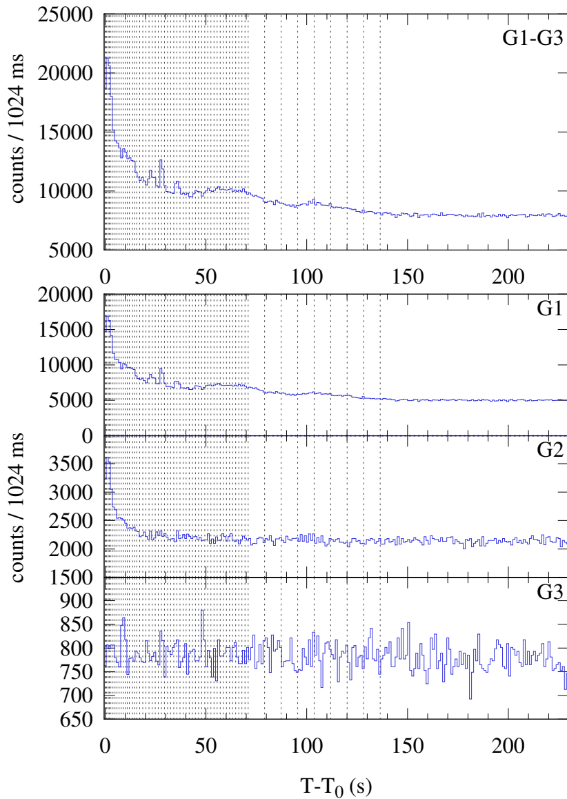
Konus-WIND S2 SOL2024-03-25T06:43 (M4.4) T_0 = 24198.517 s UT (06:43:18.517)
