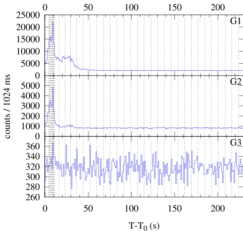
Konus-WIND S2 SOL2024-03-26T00:35 (M1.8) T 0 = 2128.123 s UT (00:35:28.123)
