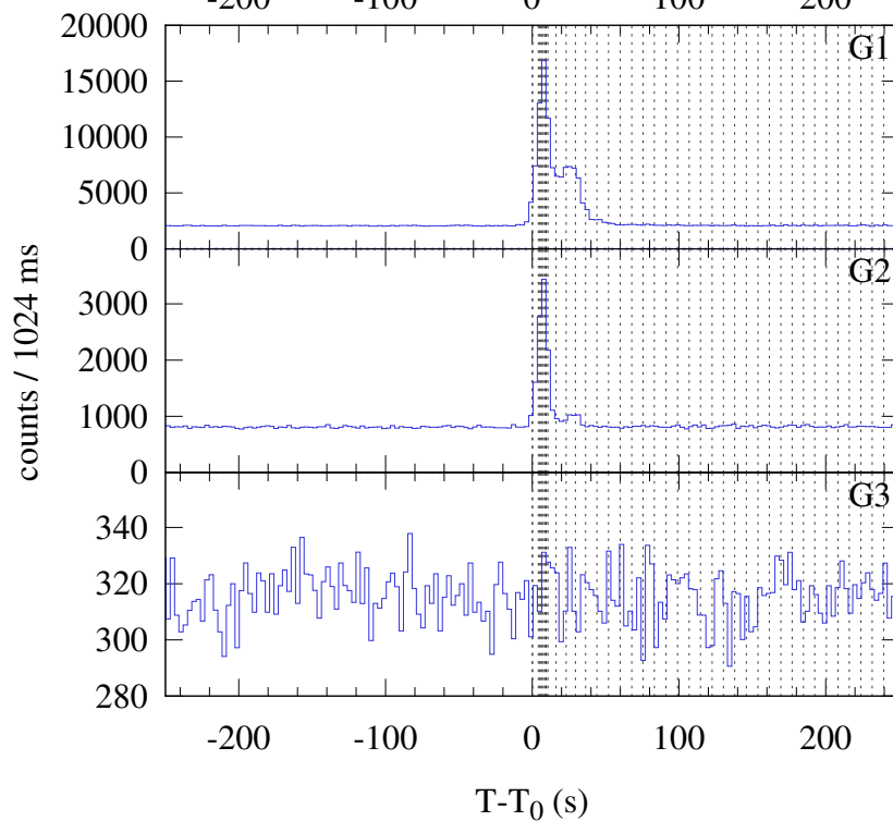
Konus-WIND S2 SOL2024-03-26T00:35 (M1.8) T 0 = 2128.123 s UT (00:35:28.123)
