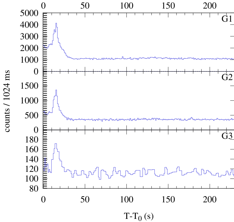
Konus-WIND S2 SOL2024-04-12T17:52 (C8.9) T_0 = 64357.175 s UT (17:52:37.175)
