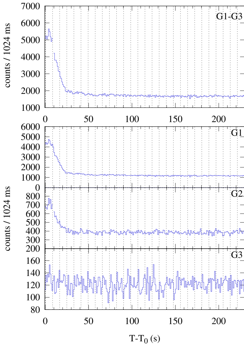
Konus-WIND S2 SOL2024-04-15T08:40 (M2.3) T_0 = 31250.233 s UT (08:40:50.233)
