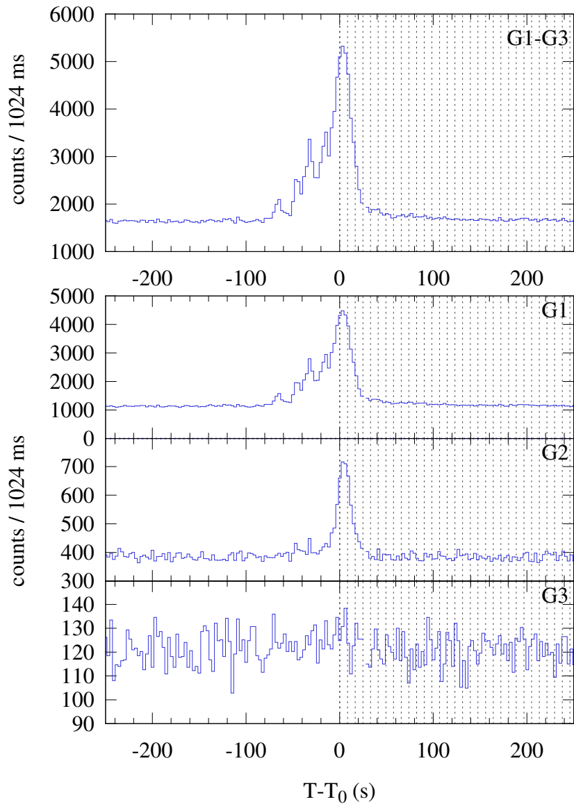
Konus-WIND S2 SOL2024-04-15T08:40 (M2.3) T_0 = 31250.233 s UT (08:40:50.233)
