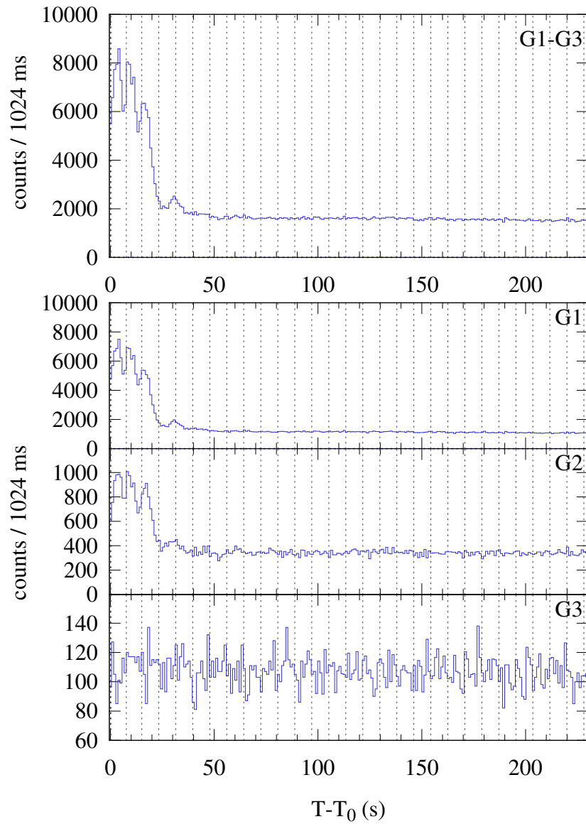
Konus-WIND S2 SOL2024-04-21T15:11 (M2.2) T 0 = 54683.949 s UT (15:11:23.949)
