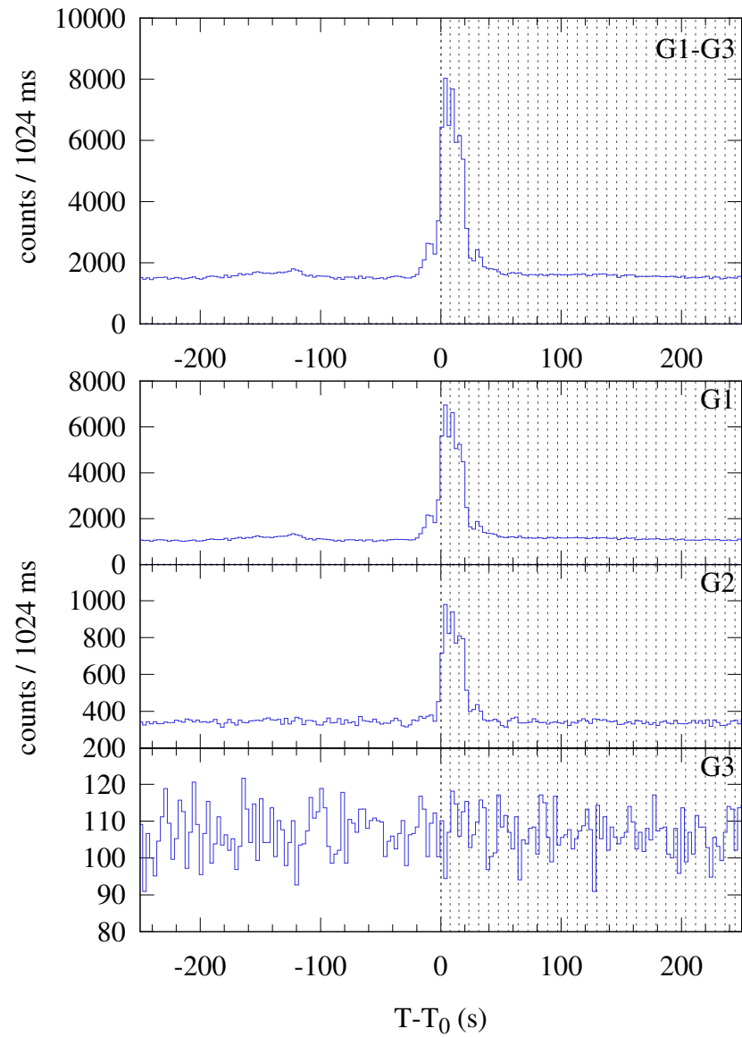
Konus-WIND S2 SOL2024-04-21T15:11 (M2.2) T 0 = 54683.949 s UT (15:11:23.949)
