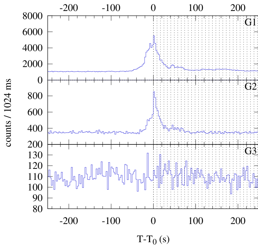
Konus-WIND S2 SOL2024-04-21T21:48 (M3.4) T_0 = 78512.252 s UT (21:48:32.252)
