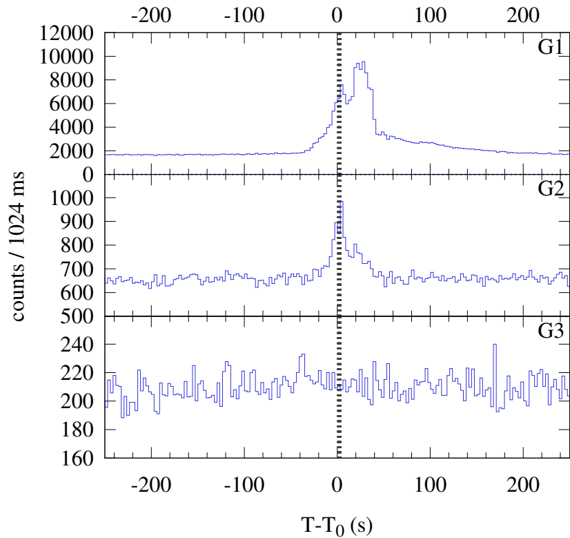
Konus-WIND S2 SOL2024-05-09T13:20 (M3.7) T_0 = 48009.249 s UT (13:20:09.249)
