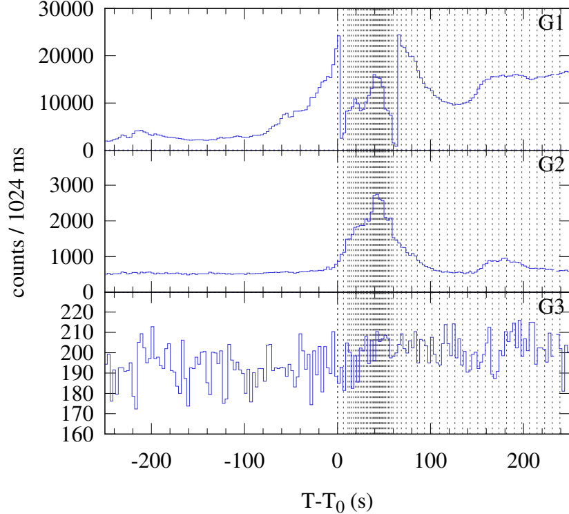
Konus-WIND S2 SOL2024-05-10T06:42 (X3.9) T 0 = 24141.646 s UT (06:42:21.646)
