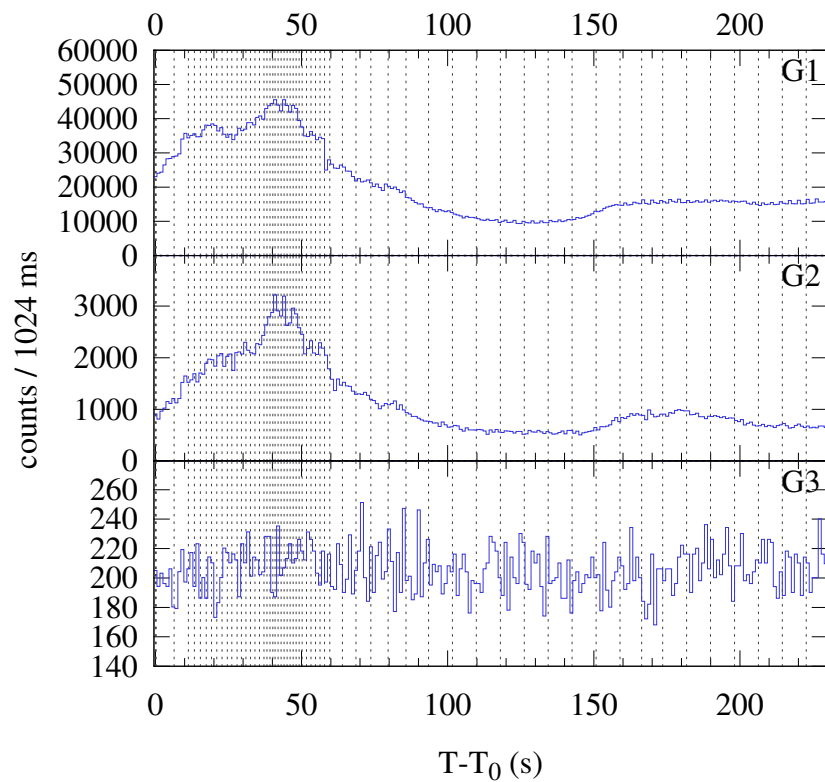
Konus-WIND S2 SOL2024-05-10T06:42 (X3.9) T 0 = 24141.646 s UT (06:42:21.646)
