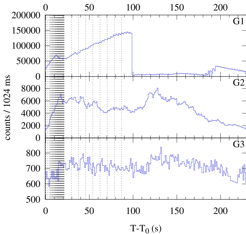
Konus-WIND S2 SOL2024-05-14T16:46 (X8.7) T_0 = 60399.537 s UT (16:46:39.537)
