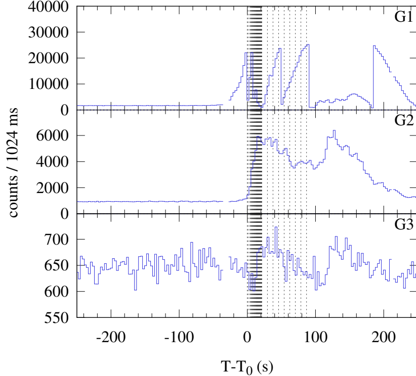
Konus-WIND S2 SOL2024-05-14T16:46 (X8.7) T_0 = 60399.537 s UT (16:46:39.537)
