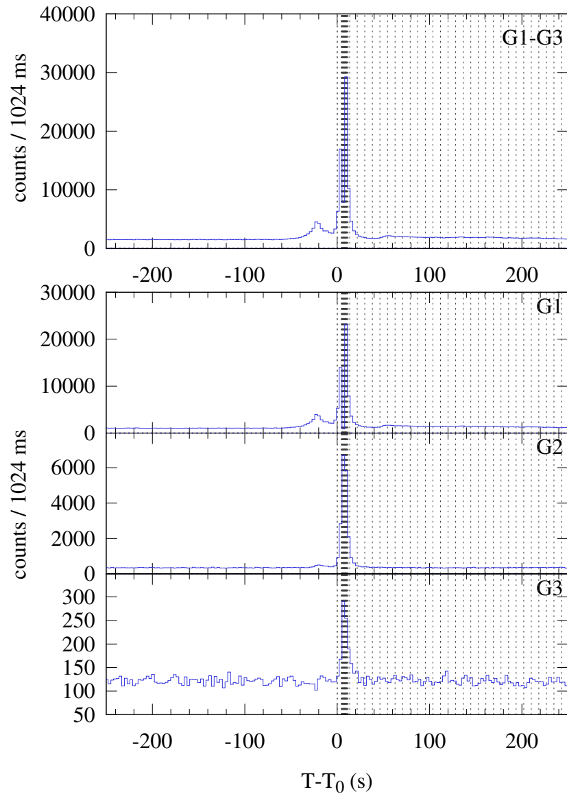
Konus-WIND S2 SOL2024-06-03T11:52 (M3.2) T_0 = 42742.688 s UT (11:52:22.688)
