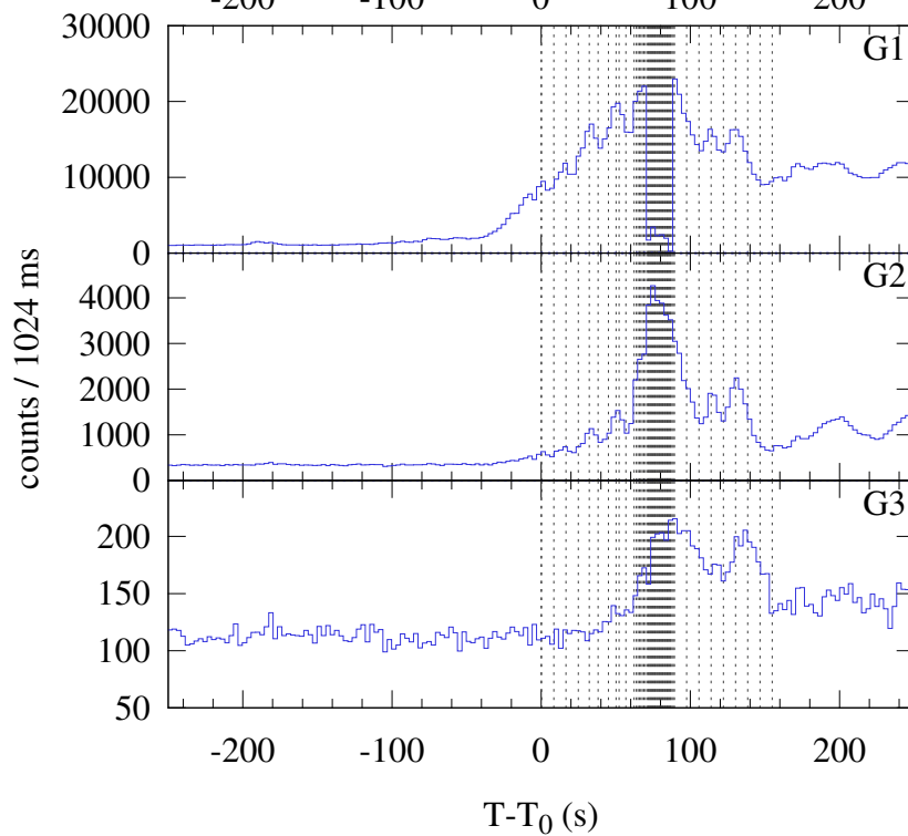
Konus-WIND S2 SOL2024-07-16T13:18 (X1.9) T_0 = 47930.52 s UT (13:18:50.52)
