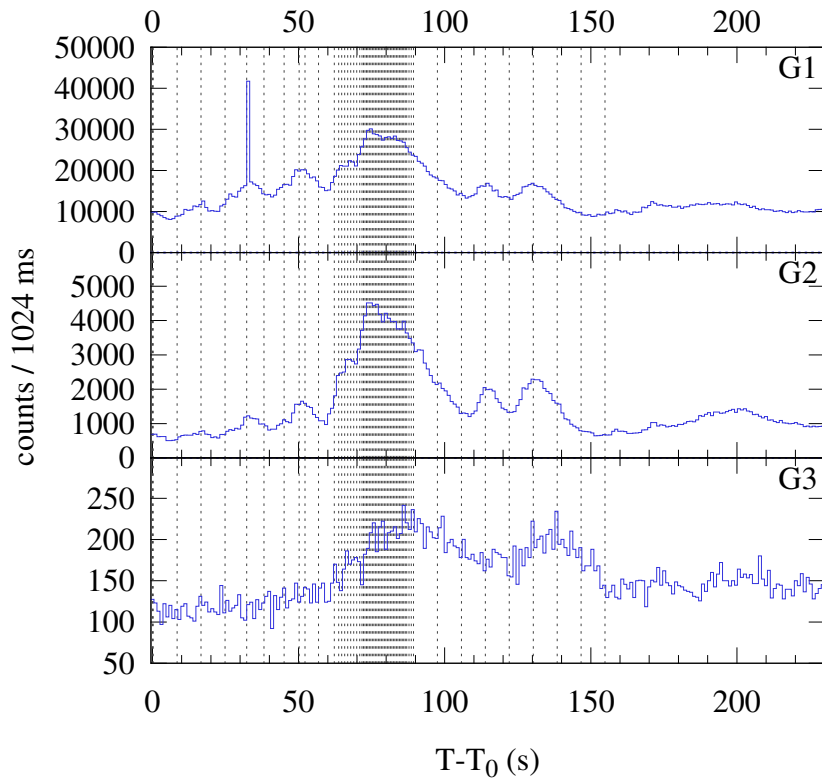
Konus-WIND S2 SOL2024-07-16T13:18 (X1.9) T_0 = 47930.52 s UT (13:18:50.52)
