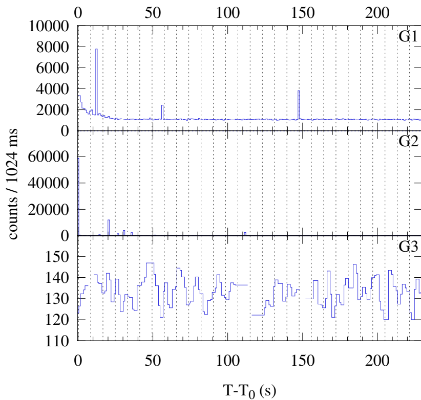
Konus-WIND S2 SOL2024-07-22T06:55 (C6.2) T_0 = 24921.930 s UT (06:55:21.930)
