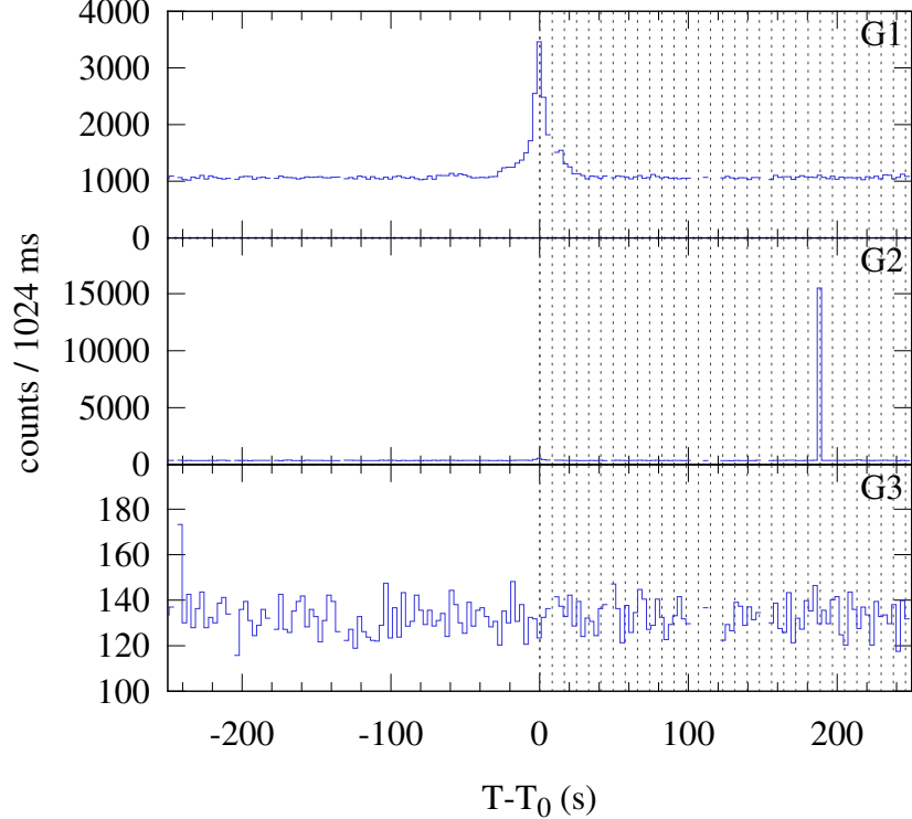
Konus-WIND S2 SOL2024-07-22T06:55 (C6.2) T_0 = 24921.930 s UT (06:55:21.930)
