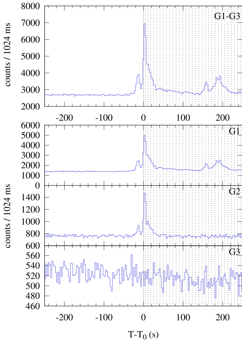
Konus-WIND S2 SOL2024-07-24T07:34 (M3.6) T_0 = 27254.951 s UT (07:34:14.951)
