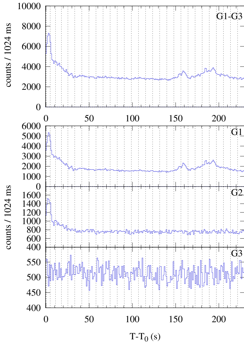
Konus-WIND S2 SOL2024-07-24T07:34 (M3.6) T_0 = 27254.951 s UT (07:34:14.951)
