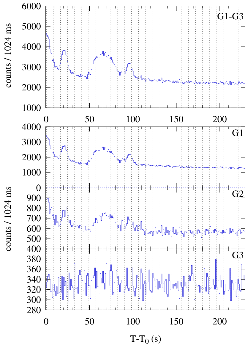
Konus-WIND S2 SOL2024-07-24T17:17 (M2.9) T_0 = 62242.264 s UT (17:17:22.264)
