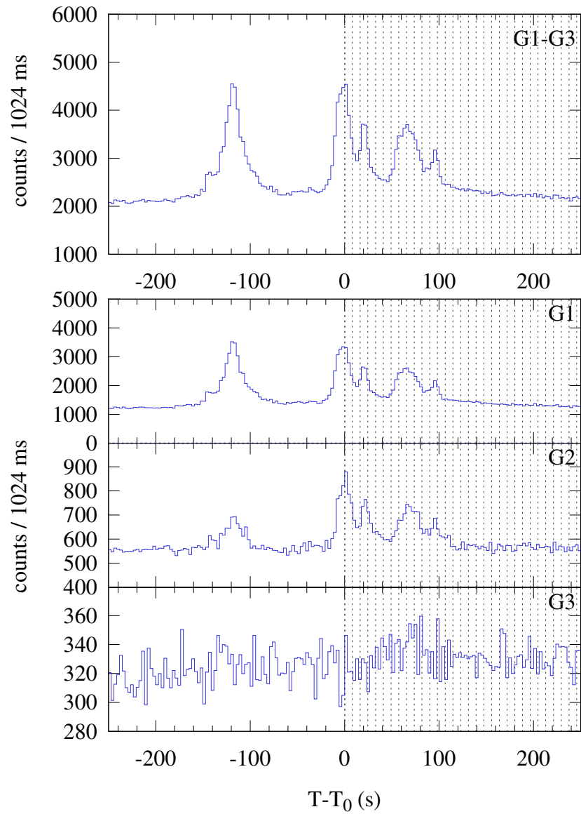
Konus-WIND S2 SOL2024-07-24T17:17 (M2.9) T_0 = 62242.264 s UT (17:17:22.264)
