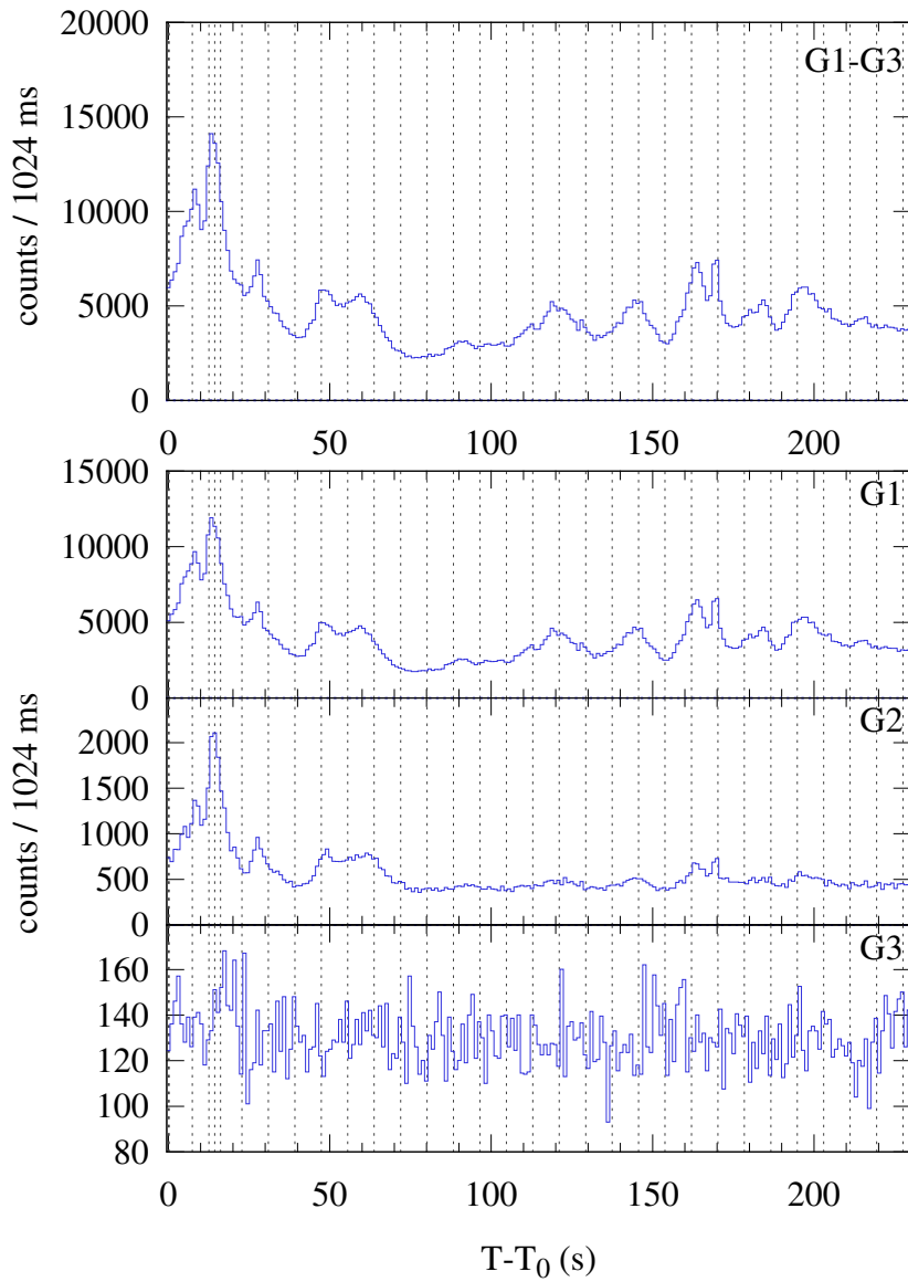
Konus-WIND S2 SOL2024-07-28T01:49 (M7.8) T_0 = 6558.567 s UT (01:49:18.567)
