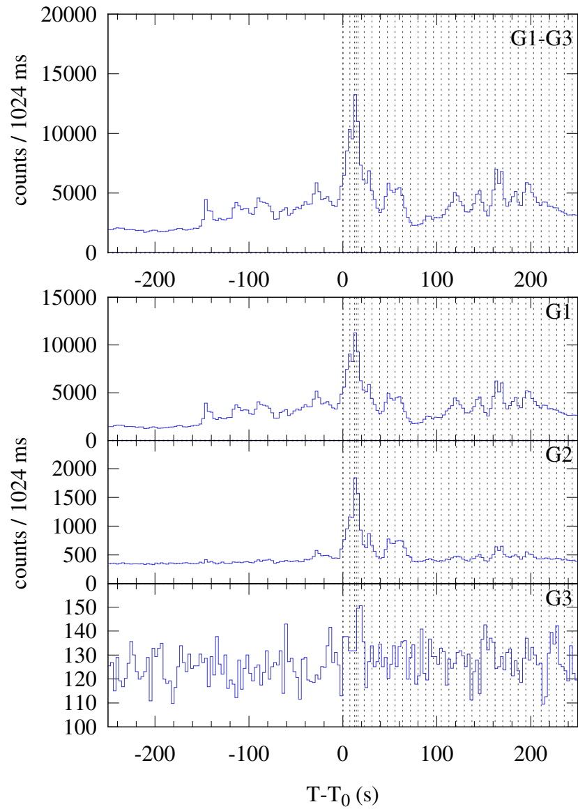
Konus-WIND S2 SOL2024-07-28T01:49 (M7.8) T_0 = 6558.567 s UT (01:49:18.567)
