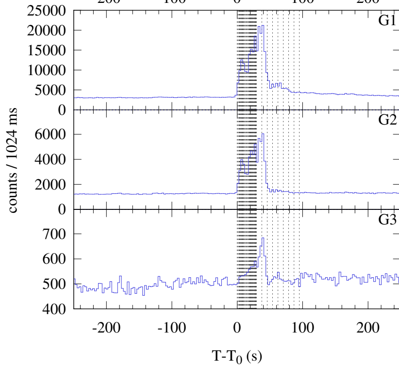
Konus-WIND S2 SOL2024-08-01T01:47 (M6.3) T_0 = 6425.574 s UT (01:47:05.574)
