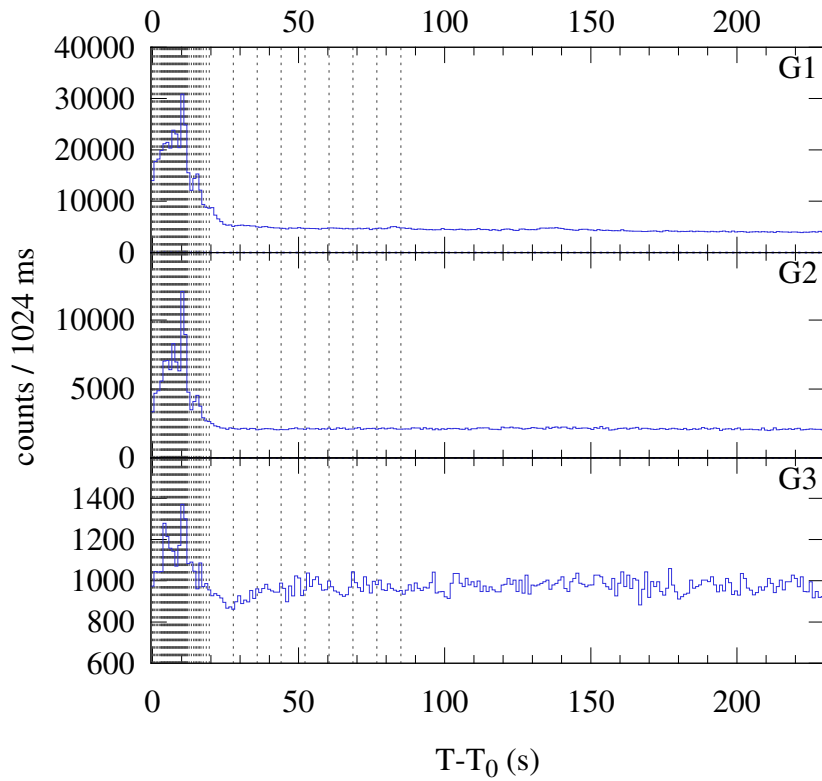
Konus-WIND S2 SOL2024-08-01T04:39 (M4.0) T_0 = 16773.555 s UT (04:39:33.555)
