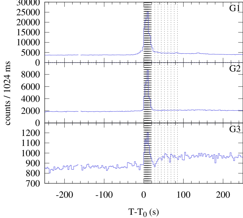
Konus-WIND S2 SOL2024-08-01T04:39 (M4.0) T_0 = 16773.555 s UT (04:39:33.555)
