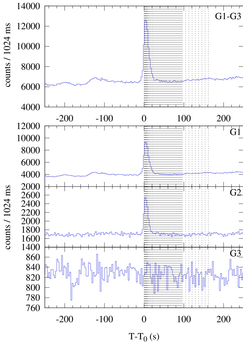
Konus-WIND S2 SOL2024-08-01T07:01 (M8.2) T_0 = 25315.916 s UT (07:01:55.916)
