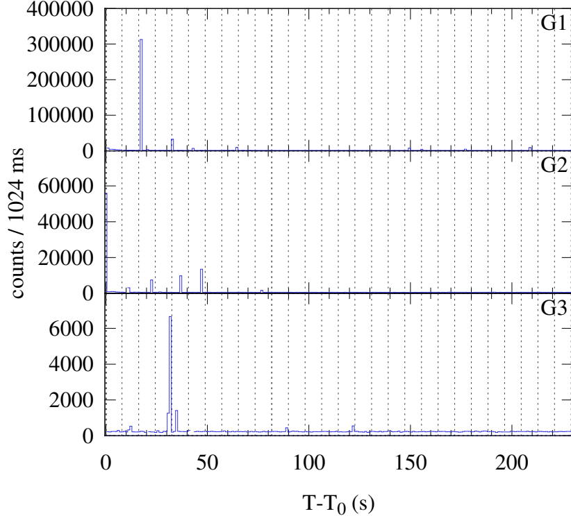
Konus-WIND S2 SOL2024-08-01T20:20 (M1.2) T_0 = 73208.330 s UT (20:20:08.330)
