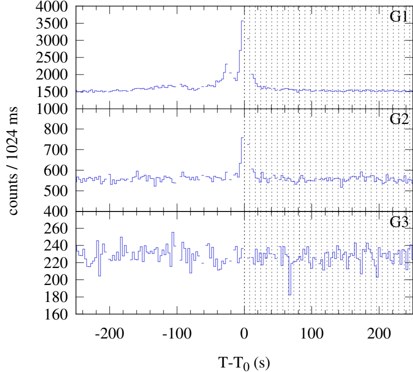
Konus-WIND S2 SOL2024-08-01T20:20 (M1.2) T_0 = 73208.330 s UT (20:20:08.330)
