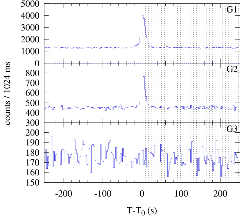
Konus-WIND S2 SOL2024-08-02T07:57 (M2.1) T_0 = 28667.321 s UT (07:57:47.321)
