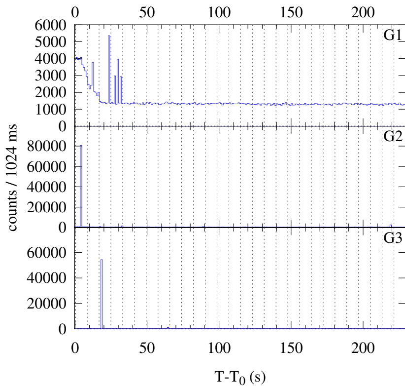
Konus-WIND S2 SOL2024-08-02T07:57 (M2.1) T_0 = 28667.321 s UT (07:57:47.321)
