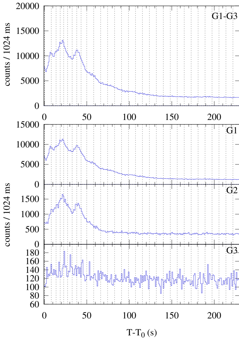
Konus-WIND S2 SOL2024-08-03T18:37 (M7.3) T_0 = 67054.598 s UT (18:37:34.598)
