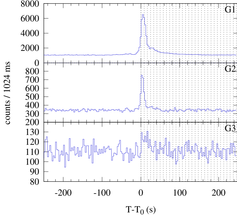
Konus-WIND S2 SOL2024-08-04T15:13 (M2.2) T_0 = 54807.600 s UT (15:13:27.600)
