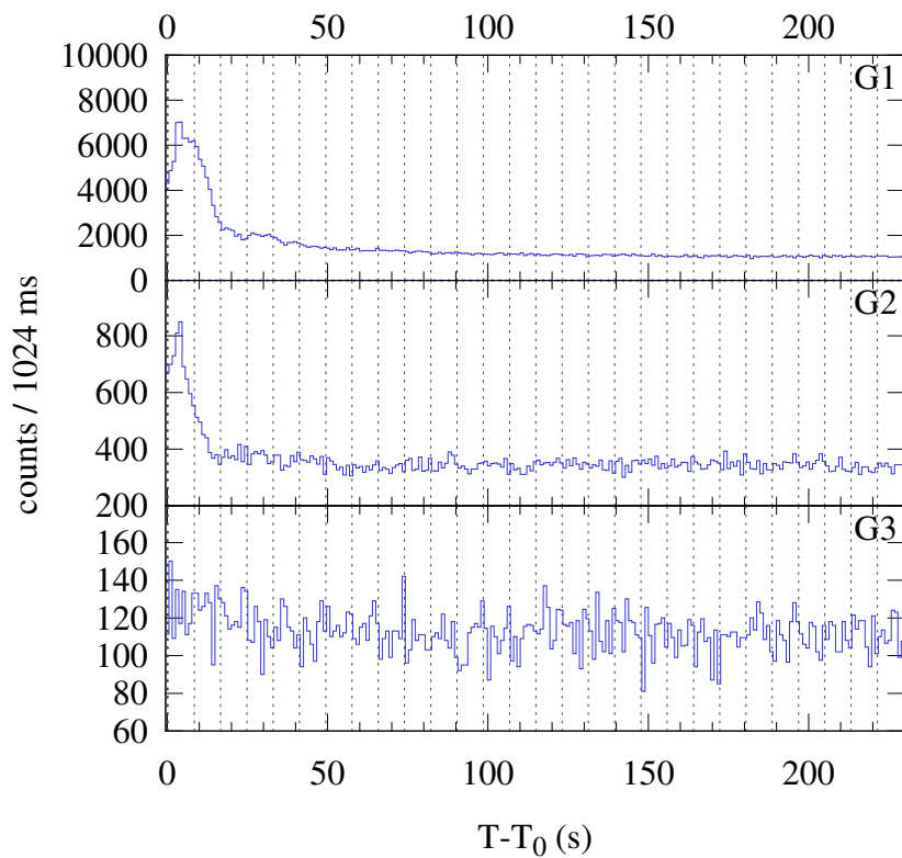
Konus-WIND S2 SOL2024-08-04T15:13 (M2.2) T_0 = 54807.600 s UT (15:13:27.600)
