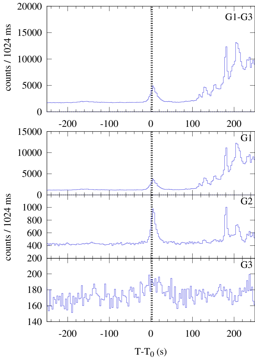
Konus-WIND S2 SOL2024-08-05T15:23 (X1.1) T 0 = 55382.400 s UT (15:23:02.400)
