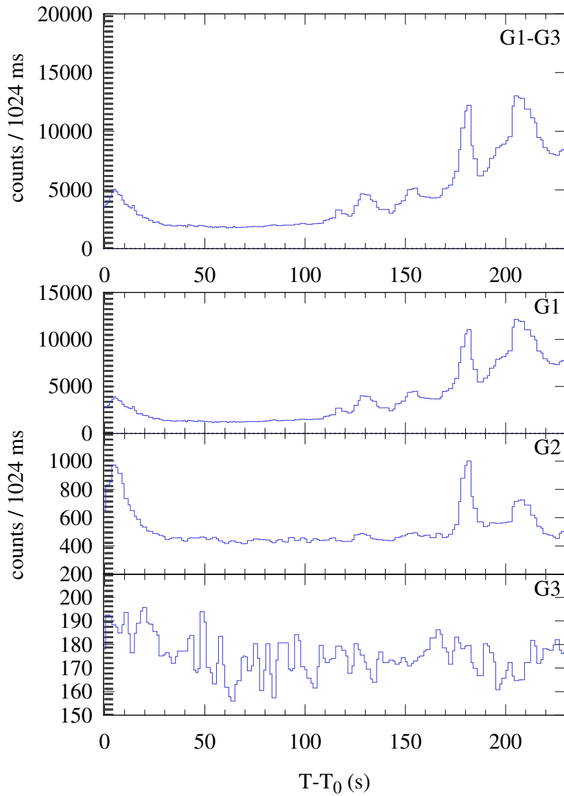
Konus-WIND S2 SOL2024-08-05T15:23 (X1.1) T 0 = 55382.400 s UT (15:23:02.400)
