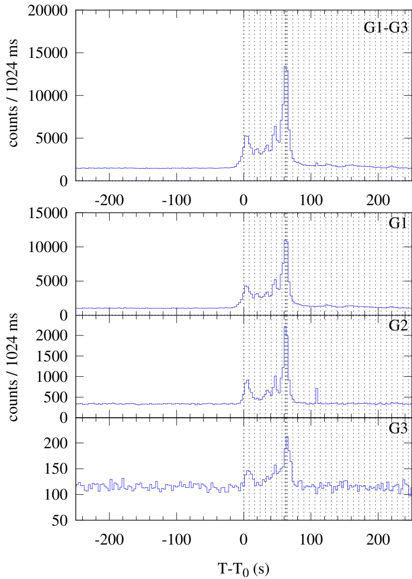
Konus-WIND S2 SOL2024-08-23T03:37 (M3.4) T_0 = 13075.144 s UT (03:37:55.144)
