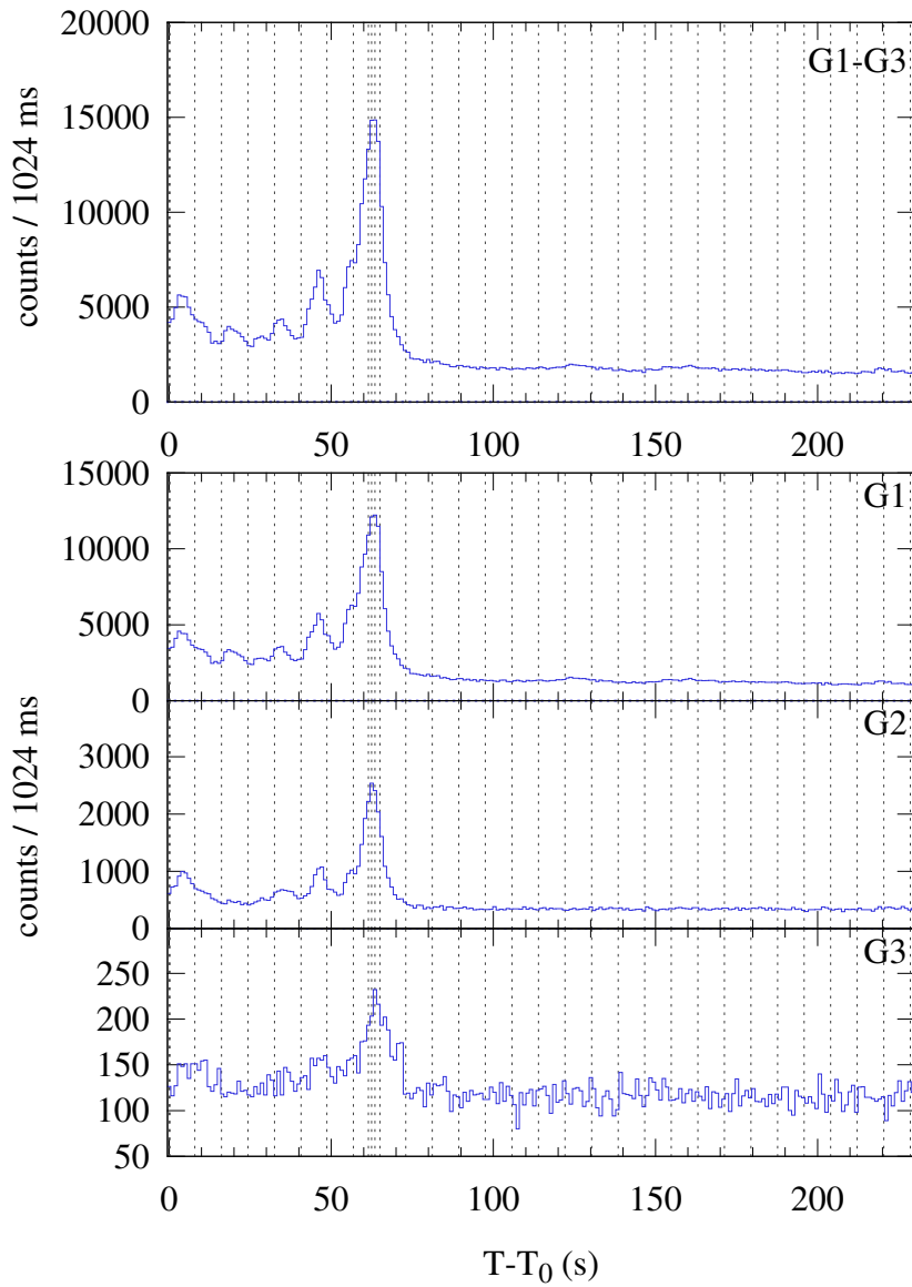
Konus-WIND S2 SOL2024-08-23T03:37 (M3.4) T_0 = 13075.144 s UT (03:37:55.144)
