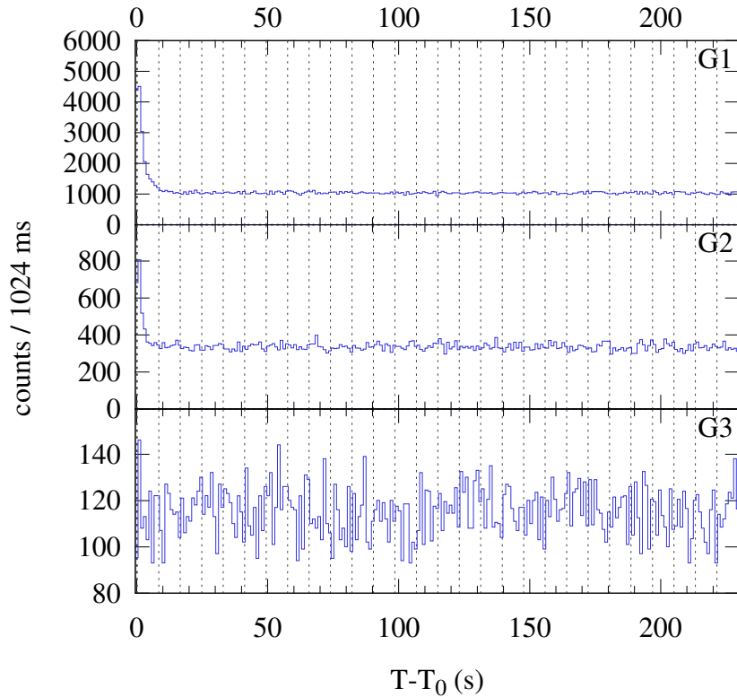
Konus-WIND S2 SOL2024-08-23T05:40 (C5.2) T_0 = 20459.187 s UT (05:40:59.187)
