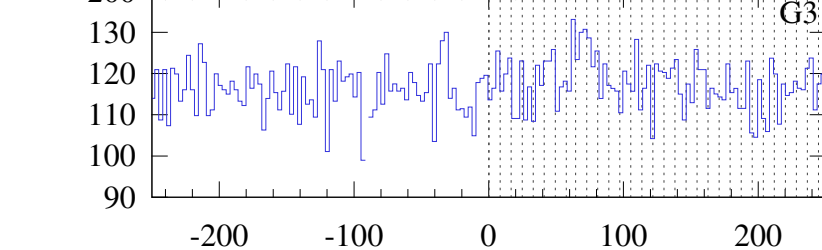
Konus-WIND S2 SOL2024-08-30T12:18 (M3.8) T_0 = 44292.770 s UT (12:18:12.770)
