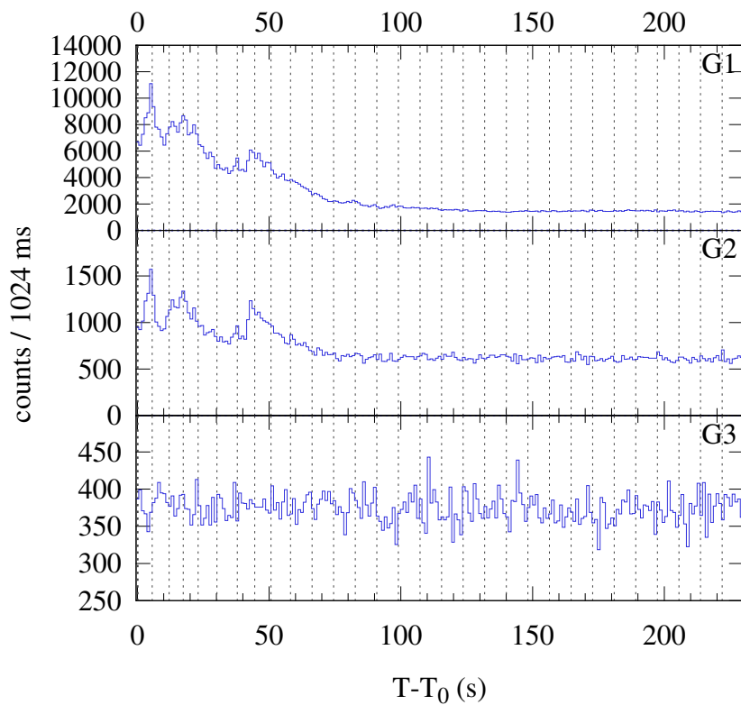
Konus-WIND S2 SOL2024-09-04T02:50 (M1.4) T_0 = 10236.68 s UT (02:50:36.68)
