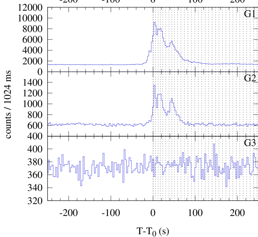
Konus-WIND S2 SOL2024-09-04T02:50 (M1.4) T_0 = 10236.68 s UT (02:50:36.68)
