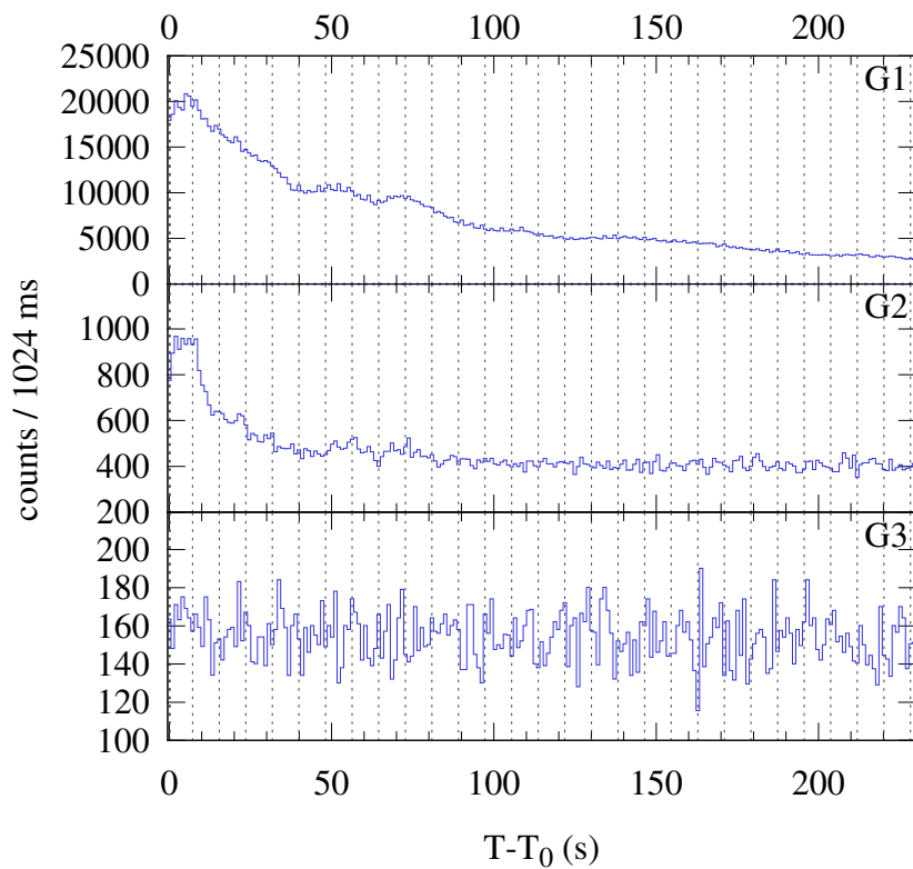
Konus-WIND S2 SOL2024-09-12T09:39 (X1.3) T_0 = 34793.867 s UT (09:39:53.867)
