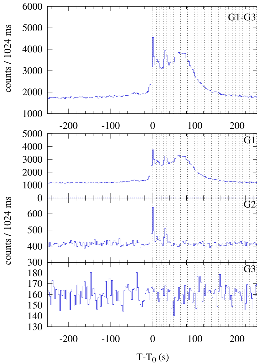
Konus-WIND S2 SOL2024-09-12T14:41 (M6.8) T_0 = 52890.419 s UT (14:41:30.419)
