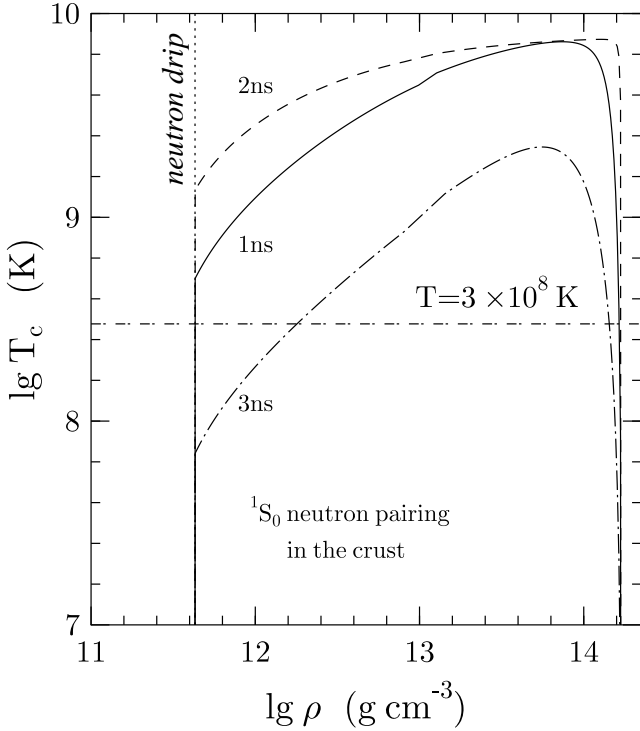
Fig. 4. Density dependence of the critical temperatures of superfluidity of neutrons (models 1ns, 2ns, and 3ns) in the NS crust (cf. Fig. 1). Vertical dotted line indicates neutron drip point. Horizontal line is the temperature of matter, T = 3 \times 10^8 K, adopted in Fig. 5.
