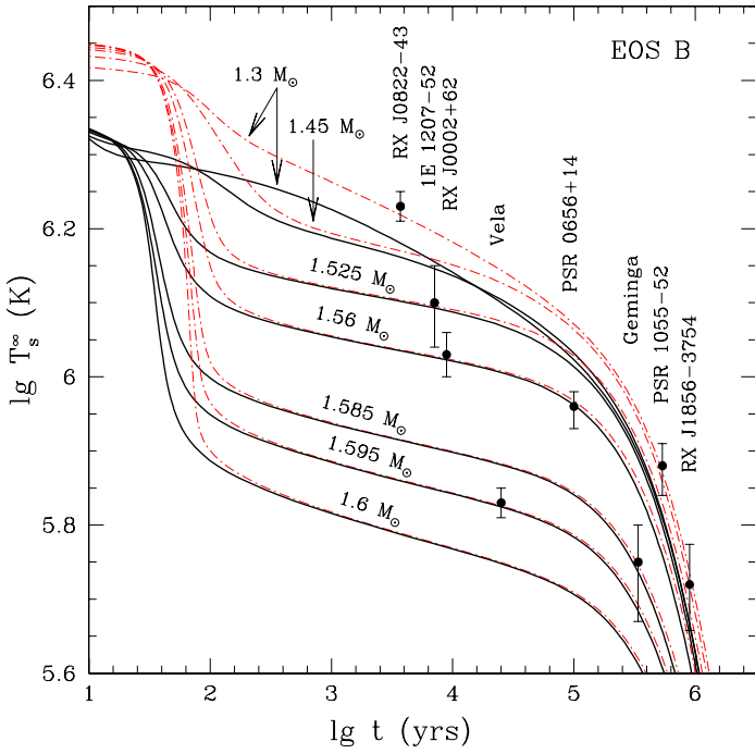
Fig. 11. Observational limits on surface temperatures of NSs compared with cooling curves of NSs (EOS B) with masses from 1.3 to 1.6 M_{\odot} (from KYG). Dot-and-dashed curves are obtained using model 3p of proton superfluidity. Solid curves include, in addition, model 1ns of neutron superfluidity.
