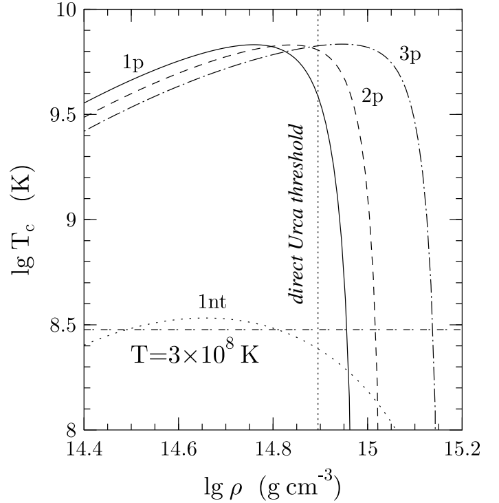
Fig. 2. Density dependence of the critical temperatures of superfluidity of protons (models 1p, 2p, and 3p — solid, dashed, and dot-and-dashed lines) and neutrons (model 1nt — dotted line) in the NS core for EOS A on a larger scale than in Fig. 1. Vertical dotted line indicates direct Urca threshold. Horizontal line is the temperature of matter, T = 3 \times 10^8 \text{ K} , adopted in Fig. 3.
