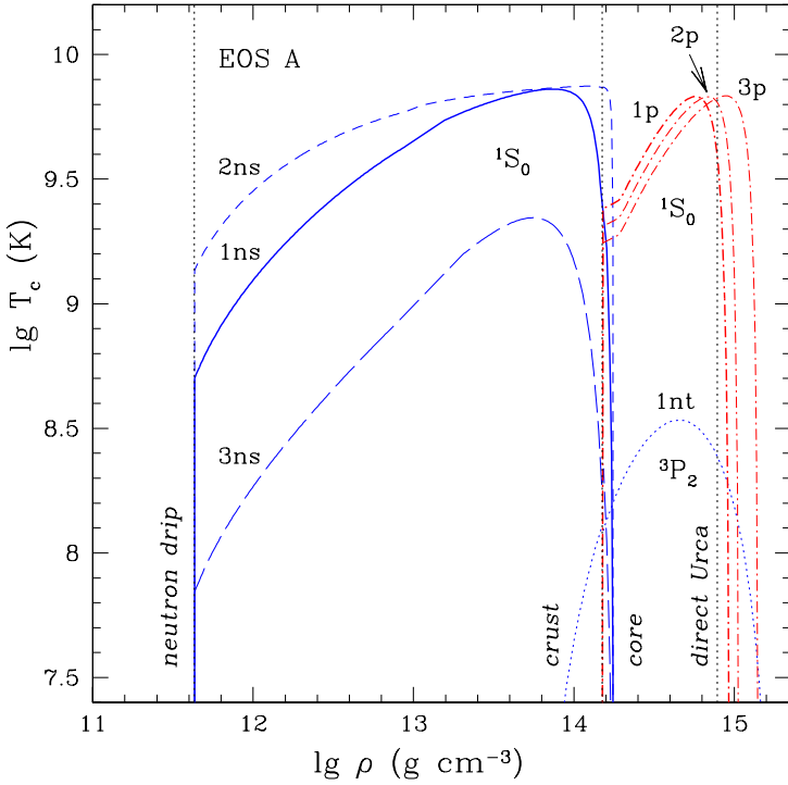
Fig. 1. Density dependence (from KYG) of the critical temperatures for three models 1p, 2p, and 3p of the proton superfluidity (dots-and-dashes) in the core (with EOS A); three models 1ns, 2ns, and 3ns of ^1S_0 neutron superfluidity (solid, short-dashed, and long-dashed lines); and one model 1nt of ^3P_2 neutron superfluidity (dots) used in cooling simulations. Vertical dotted lines indicate the neutron drip point, core-crust interface, and direct Urca threshold.
