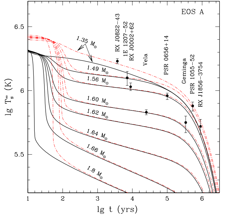
Fig. 10. Observational limits on surface temperatures of NSs compared with cooling curves of NSs (EOS A) with several masses M in the presence of proton superfluidity 2p (from KYG). Dot-and-dashed curves are obtained assuming non-superfluid neutrons. Solid curves include, in addition, model 1ns of neutron superfluidity. {}^3\text{P}_2 neutron pairing is neglected.
