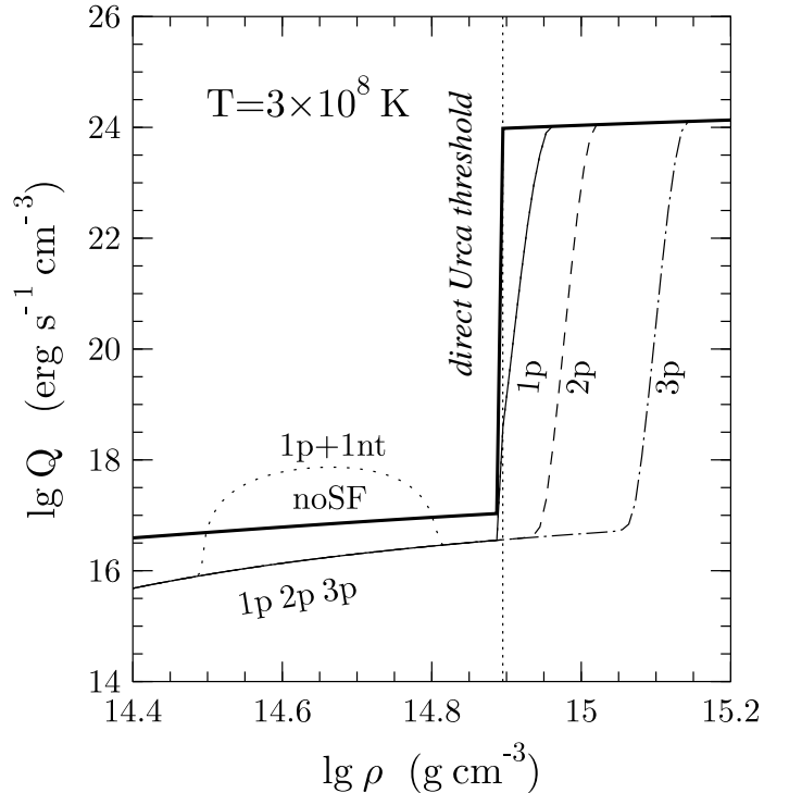
Fig. 3. Density dependence of the neutrino emissivity Q in the NS core at T = 3 \times 10^8 \text{ K} and EOS A. Solid, dashed and dot-and-dashed lines 1p, 2p, and 3p are plotted for proton superfluidity models displayed in Fig. 2. The dotted line shows Q in the presence of proton superfluidity 1p and neutron superfluidity 1nt. The thick solid line is Q in non-superfluid matter.
