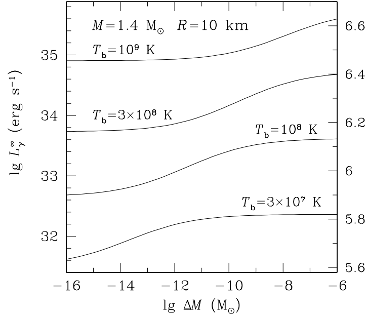
Fig. 6. Photon surface luminosity (redshifted as detected by a distant observer, left vertical axis) or redshifted effective surface temperature (right vertical axis) of a “canonical” NS model ( M = 1.4 M_\odot , R = 10 km) for four values of the “internal” temperature T_b (at the bottom of the heat blanketing layer, \rho_b = 10^{10} g cm ^{-3} ) versus the mass of accreted material, \Delta M .
