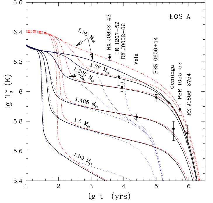
Fig. 9. Observational limits on surface temperatures of eight NSs compared with cooling curves of NSs (EOS A) with masses from 1.35 to 1.55 M_{\odot} (after KYG). Dot-and-dashed curves are obtained including proton superfluidity 1p alone. Solid curves include, in addition, model 1ns of neutron superfluidity. Dotted lines also take into account the effect of neutron superfluidity 1nt.
