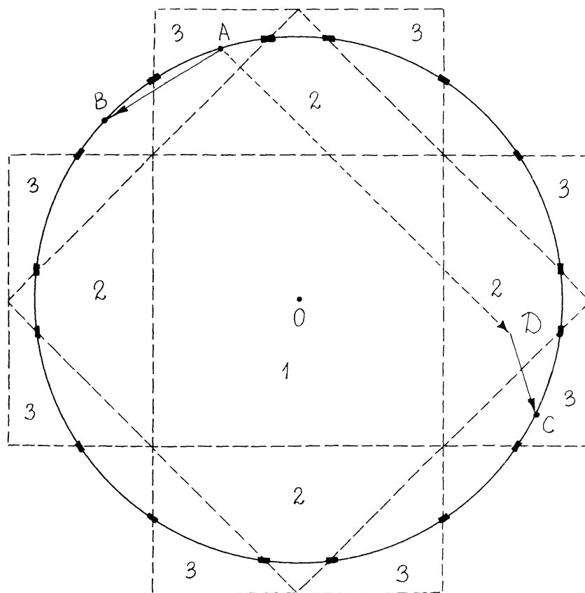
Fig. 2. A schematic picture of electron scattering on phonons in a simple square two-dimensional lattice at Z = 5 (for illustration). Dot-lines show the boundaries of the first three Brillouin zones 1, 2, and 3. The solid circle is the Fermi surface, heavy short lines indicate the places where the Fermi surface is distorted due to the Bragg reflection of electrons. The transition A \rightarrow B corresponds to normal process whereas the transition A \rightarrow C corresponds to the Umklapp process. The vectors \mathbf{AB} and \mathbf{DC} are the phonon quasi-momenta for these transitions, and \mathbf{AD} is the corresponding reciprocal cell vector for the Umklapp process.
