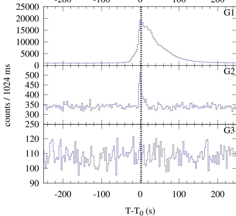
Konus-WIND S2 SOL2024-05-07T16:28 (M8.2) T_0 = 59332.907 s UT (16:28:52.907)
