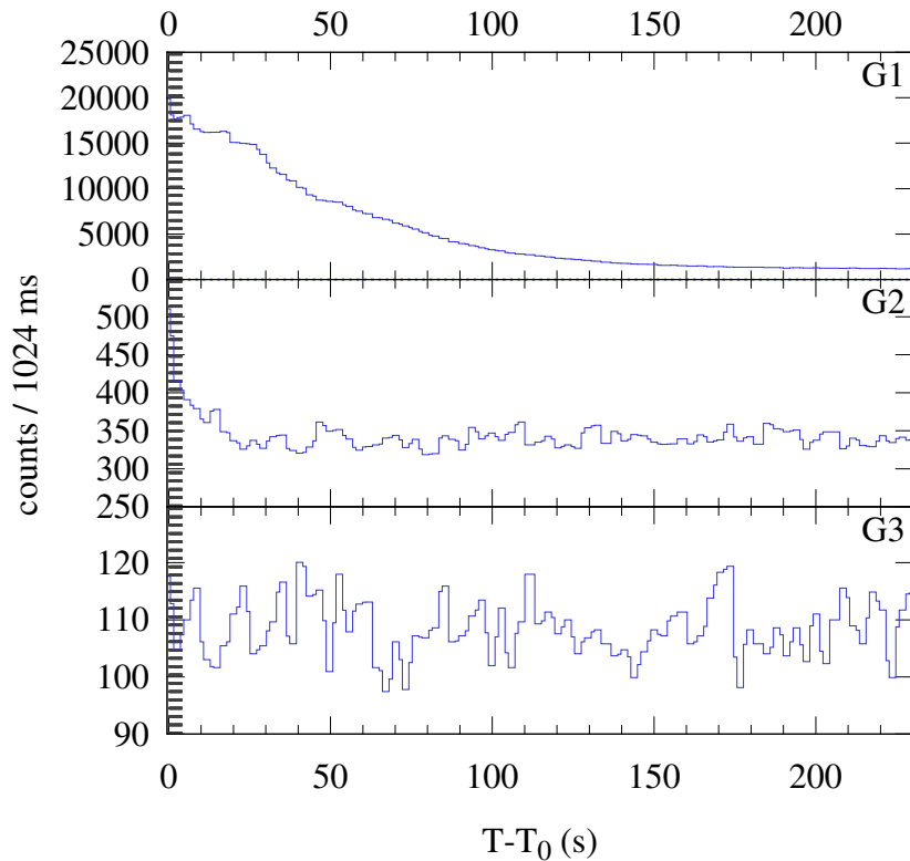
Konus-WIND S2 SOL2024-05-07T16:28 (M8.2) T_0 = 59332.907 s UT (16:28:52.907)
